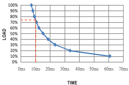
RSD-150C-5
