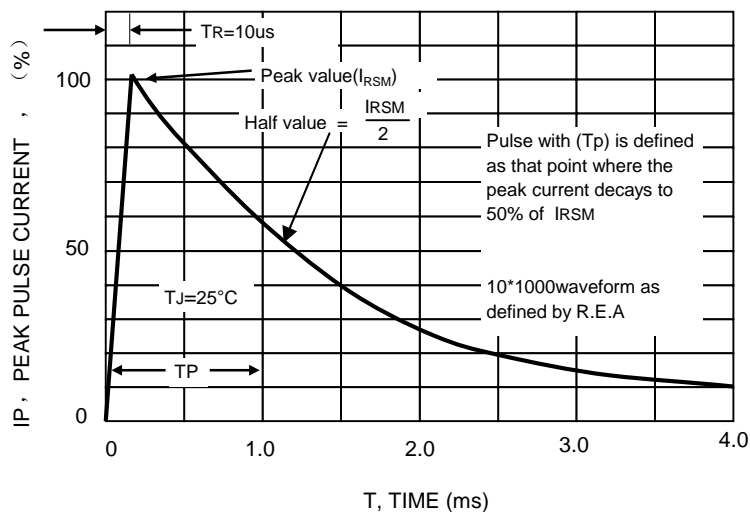
FIG.5-PULSE WAVEFORM
