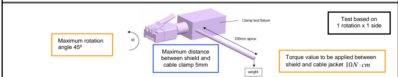
Figure 3: Torsion force test procedure
