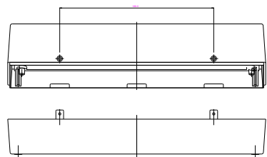
ALZADO POST. DESMONTADO REAR VIEW (OPENED)
