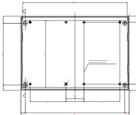
BASE: PLANTA INTERIOR BOTTOM: INSIDE VIEW
