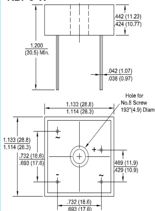
Package Outline Dimensions in Inches (Millimeters)
