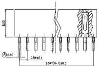
DUAL ROWS N:NUMBER OF CONTACTS/2
